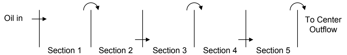
Typical Overflow/Underflow Deodorizer #1 and #2 Compartments
