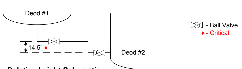
Relative height Schematic Deod #1 to Deod #2
