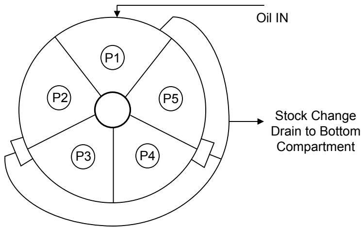
Deodorizer #1 – Top Compartment Plan View
