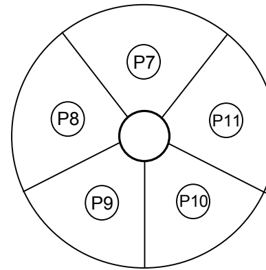
Deodorizer #2 - Plan View 5 Sections – 1 Mammoth Pump Each Thermal oil coils
